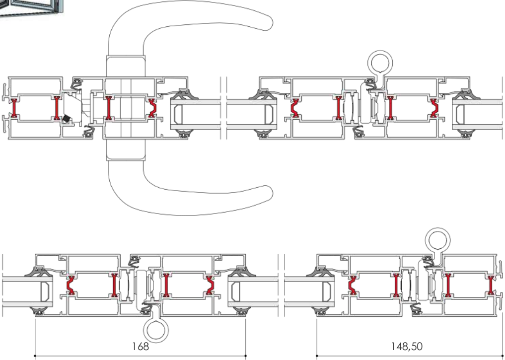
› PORTE REPLIABLE KASABI 50 HORIZONTALE
