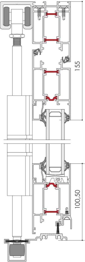
› PORTE REPLIABLE KASABI 50 VERTICALE
